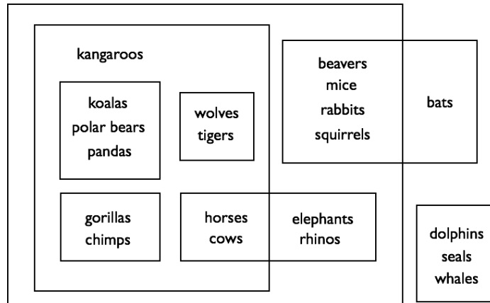
Figure 10. Visualization of the categories estimated from human inductive generalizations with the assistance of a Bayesian model. As is clear from inspection, the category structure is non-hierarchical and includes a number of cross-cutting categories.
